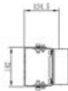
Surface Mount Bracket Dimensions (order code U2FL-SM)
